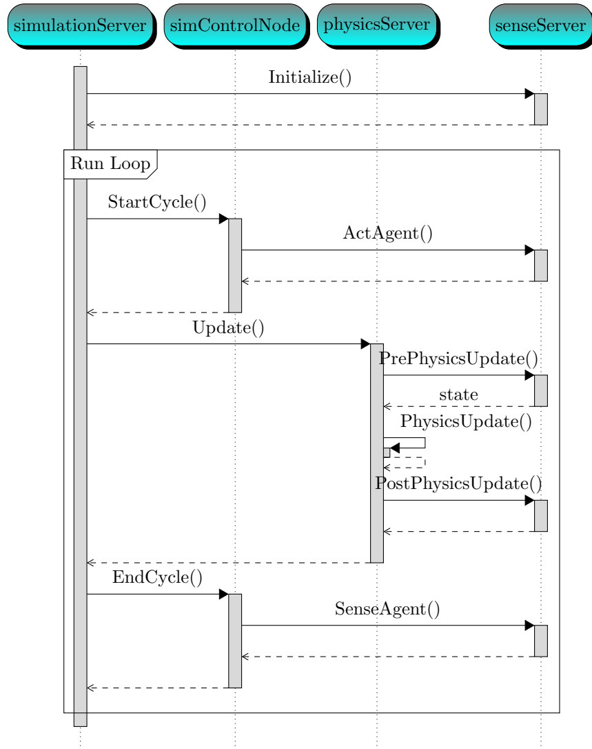
Figure 1: UML sequence diagram demo. The used style-file is part of pgf-umlstd-0.2.tar.gz Get it at http://code.google.com/p/pgf-umlstd/
