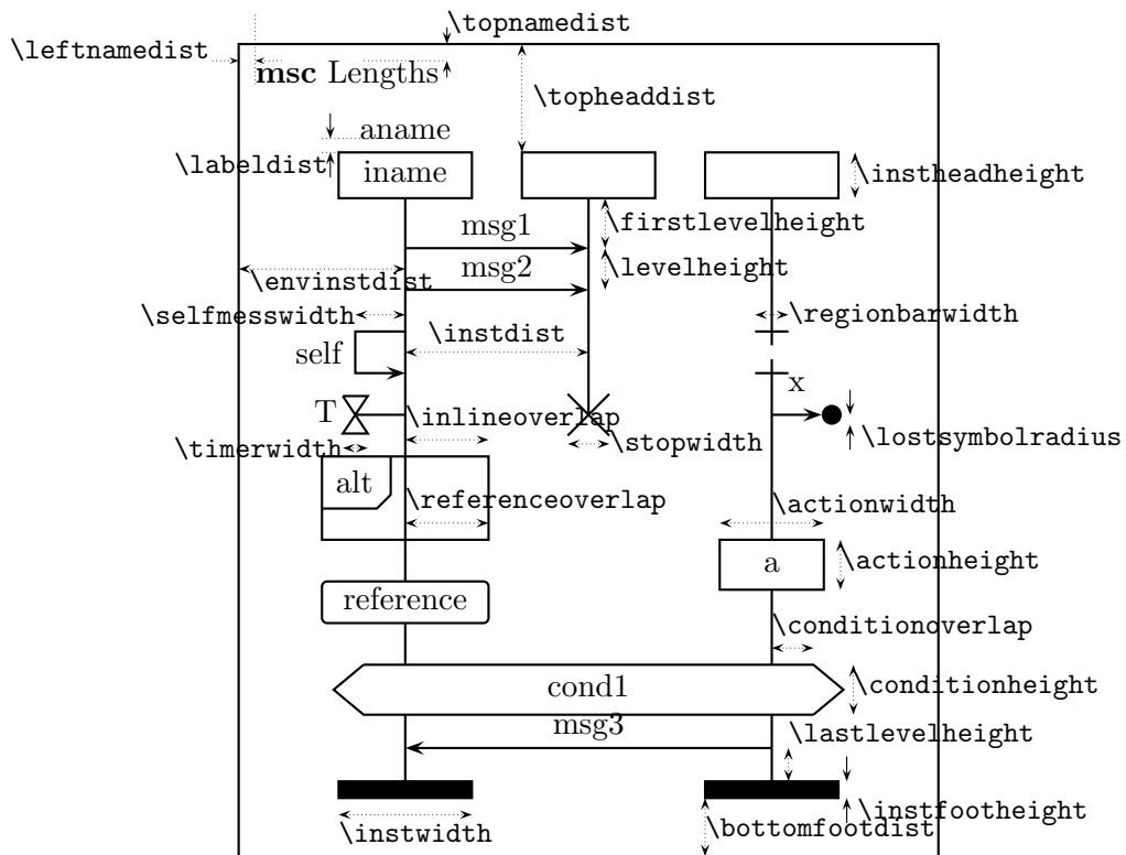
Figure 4: User controllable parameters
