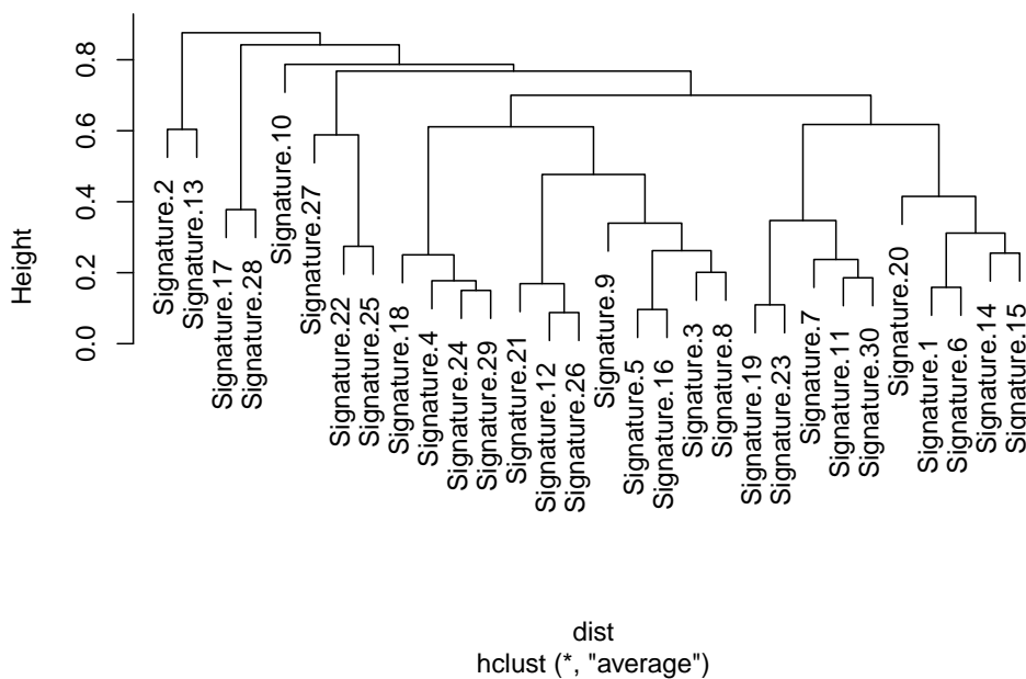
Cluster Dendrogram
