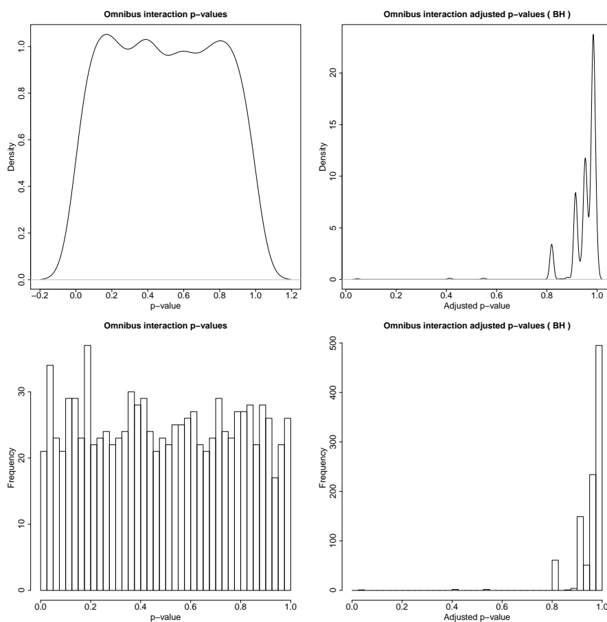
Figure 4: Assessment of whether the p-values for the interaction follow the uniform NULL distribution
