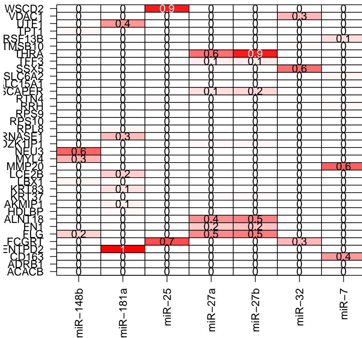
Figure 3: ProMISe generated from Section 4. Probabilities are displayed in the cells. The intensity of the red color corresponds to the magnitude of the probabilities (i.e. the higher the probability the more red).
