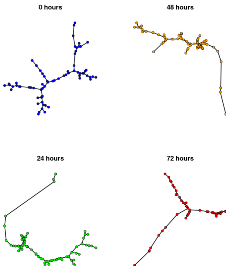
Figure 6: Cell-state hierarchies of differentiating myoblast samples at 4 time points (0, 24, 48 and 72h) obtained through a dimensionality reduction with Independent Component Analysis (ICA, 2 dimensions) and a Minimum Spanning Tree (MST)
