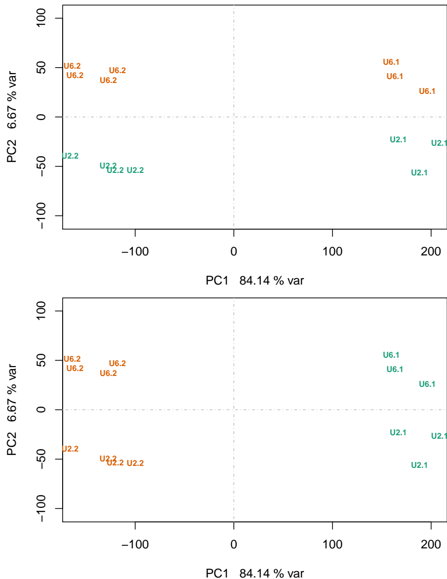
Figure 3: PCA plot on PC1/PC2, showing confounding. The labels are colored by treatment level on top, and by batch number below. Labels themselves are selfexplanatory of treatment condition and batch.
