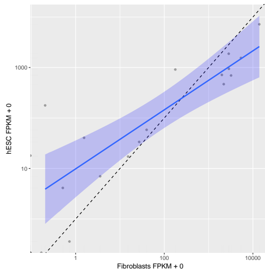
(a) Scatterplot showing relationship between two conditions for genes in a CuffGeneSet.
