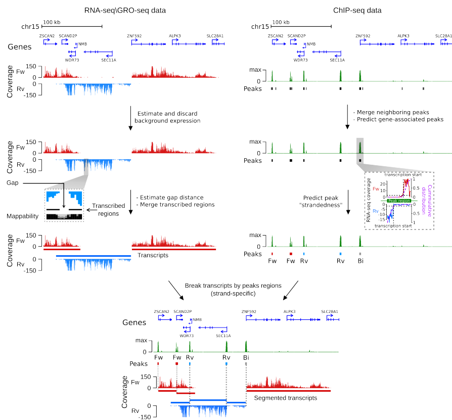
Figure 1: transcriptR workflow
