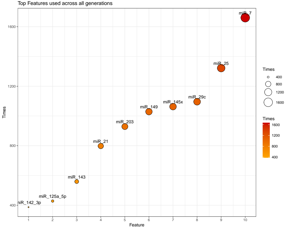
Figure 2: Recurring Features. Each circle in the plot represents a feature. The color and size of each circle are, respectively, darker and bigger when a feature is more recurring.
